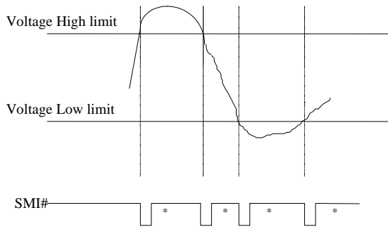
Figure 15-1. Voltage SMI# Mode
