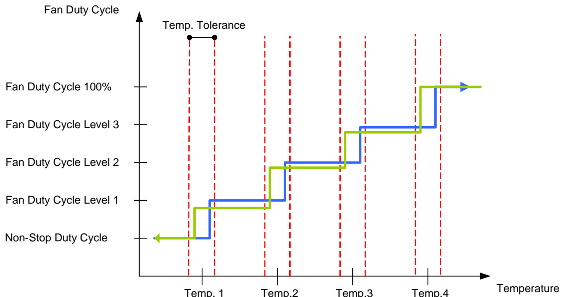
Figure 12 SMART FAN™ II behaviors
