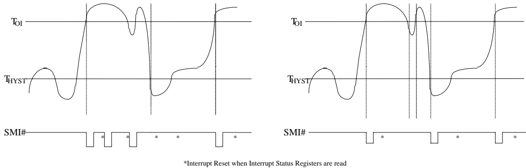
Figure 14-1. Comparator Interrupt Mode
