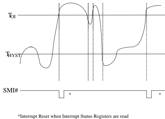
Figure 14-3. One-Time Interrupt Mode
