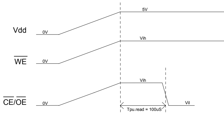
Fig.1: Power-Up to Read Operation Waveform
